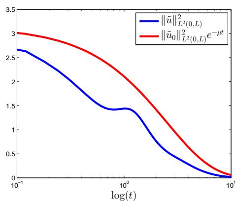
Figure 3: Logarithmic time evolution of the L^2 -norm for the observation error \tilde{u} = (u - \hat{u}) and \|\tilde{u}_0\|_{L^2(0,L)}^2 e^{-\mu t} .
